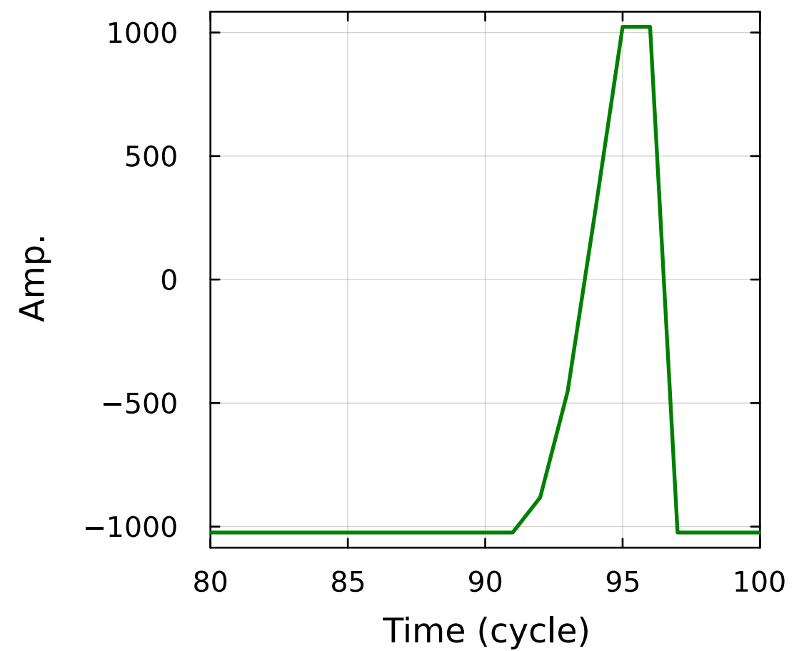
Zoom h(Zhyp=902)
