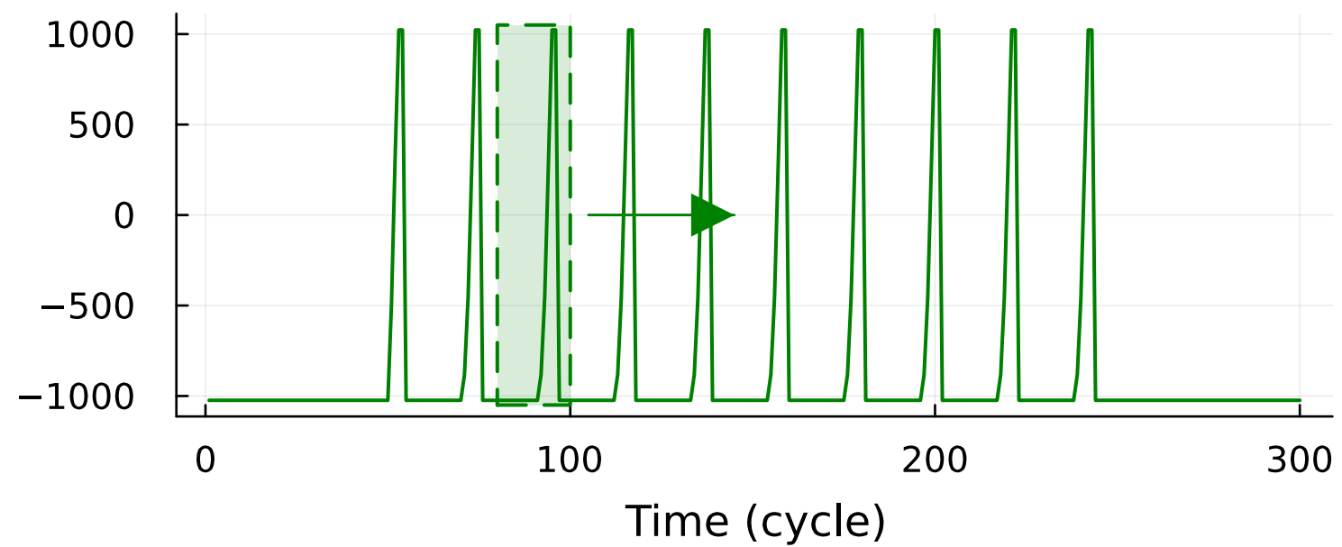
h(\text{Zhyp}=902)
