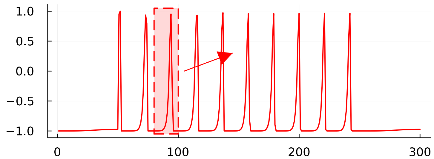
h(\text{Zhyp}=902)
