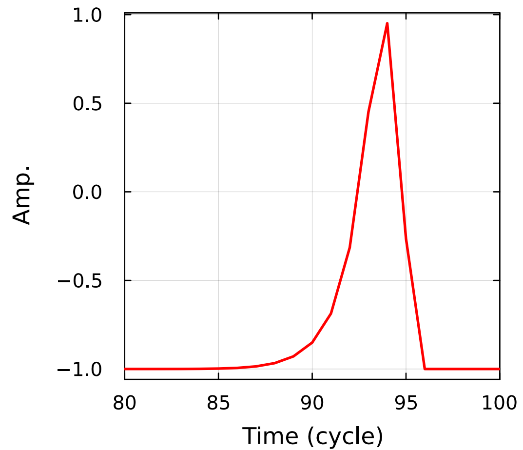
Zoom h(Zhyp=902)
