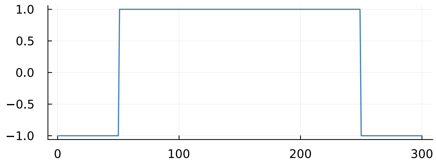
h(\text{Zhyp}=0.910)
